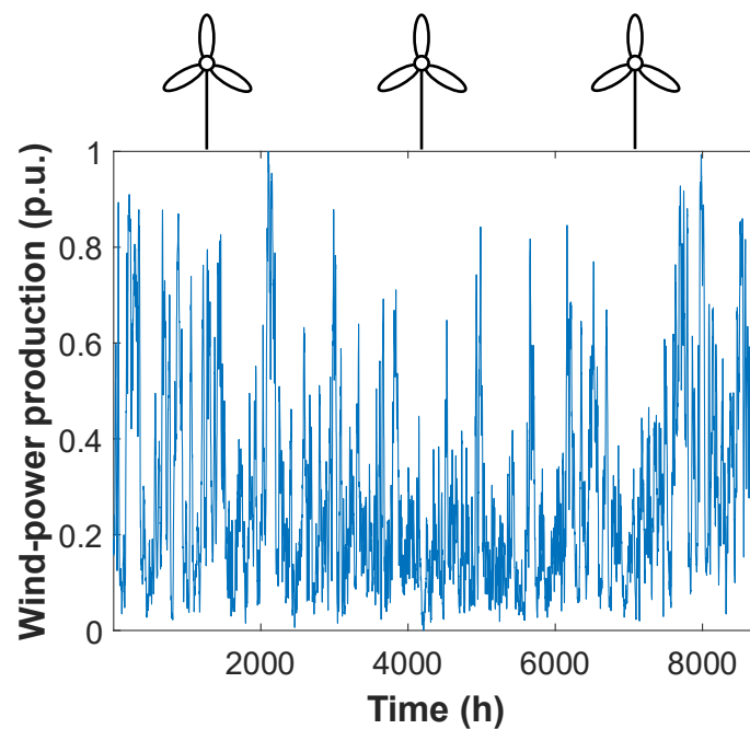
Wind-power production
